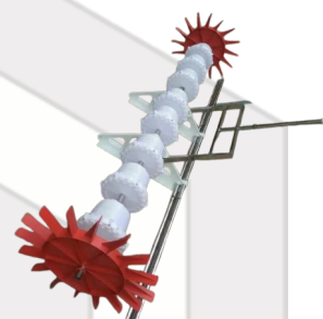
Rice Drum Seeder
