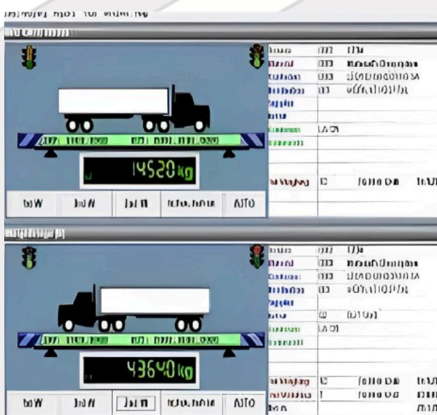
Software / Program
