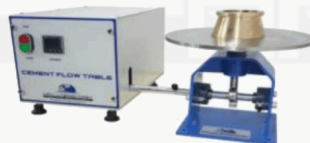
Flow Table
